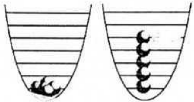
Above: Bosons are social; fermions are anti-social
