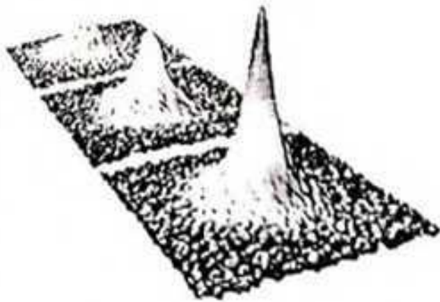
Above: Snapshots of a growing fermionic condensate
